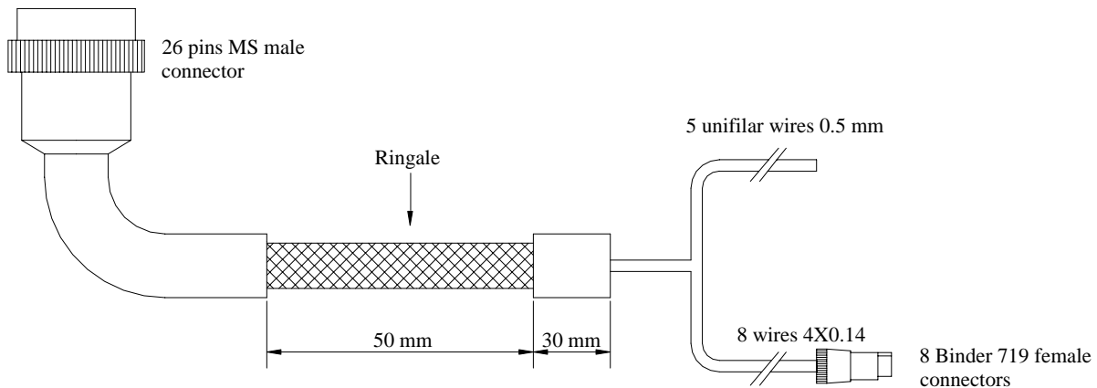
Figure 1: Dash ST1 “standalone” wiring (“no thermocouple” version)
