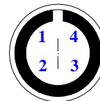
Figure 3: 4 pins female Binder connector pinout. Solder termination view
