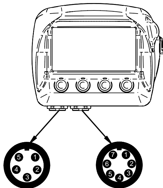
binder 5 pin female connector - pinout ext. view
