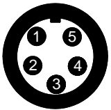
binder 5 pin female connector - pinout solder view
