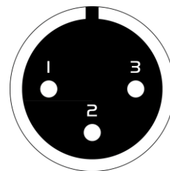
Binder 711, female, solder view
